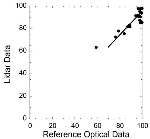
Figure 6. Comparison of the crown density between the estimation and observation
