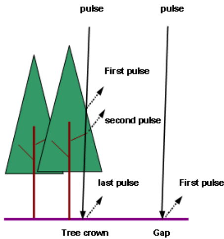
Figure 2. Multiple pulse return for the forest canopy
