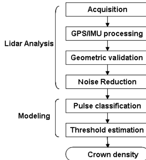
Figure 3. Flowchart of the crown density estimation algorithm
