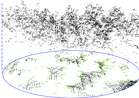
Figure 4. The distribution of the pulse of Plot 3, Hinoki (a) side view (a), and slant view (b)
